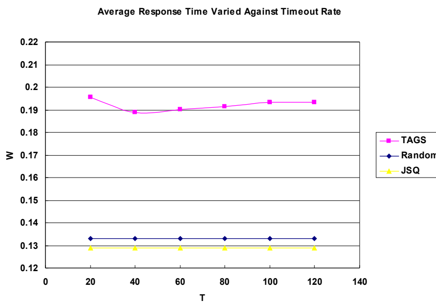
Figure 3.2 Average Response Time Varied against Timeout Rate, \lambda=5 , \mu=10
